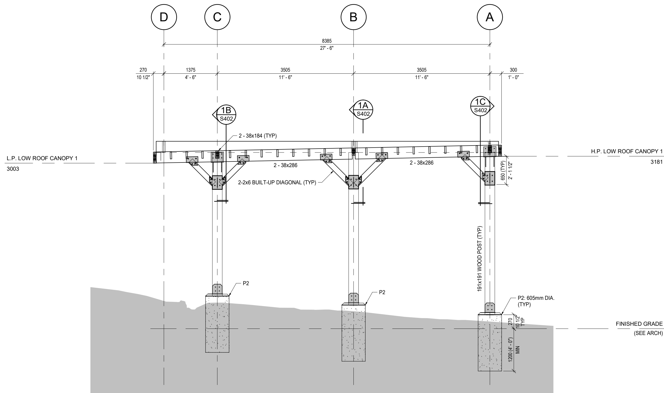
1 SECTION AT G/L 3 S401 1 : 50
