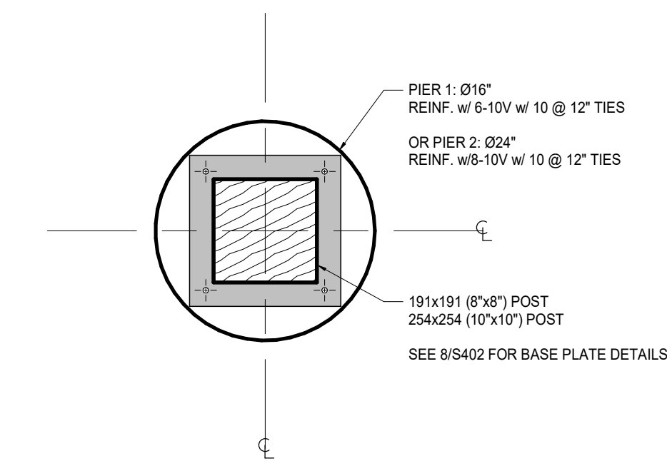
7 CONCRETE PIER & POST PLAN S402 1 : 10
