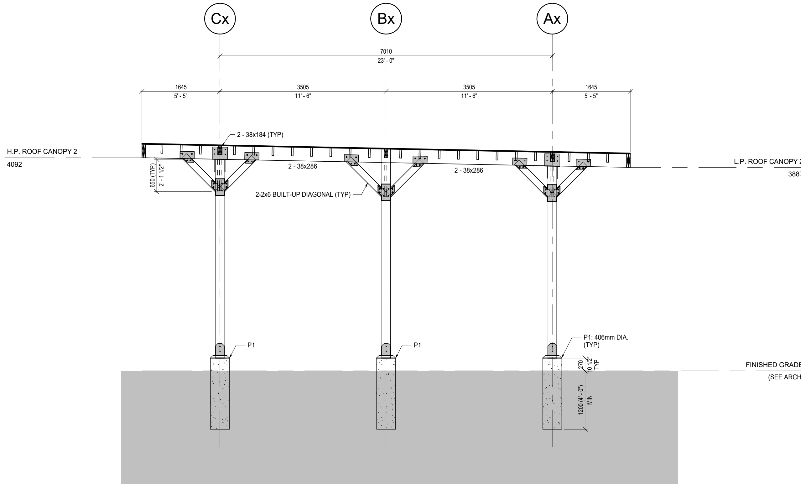
3 SECTION AT G/L 4x S401 1 : 50
