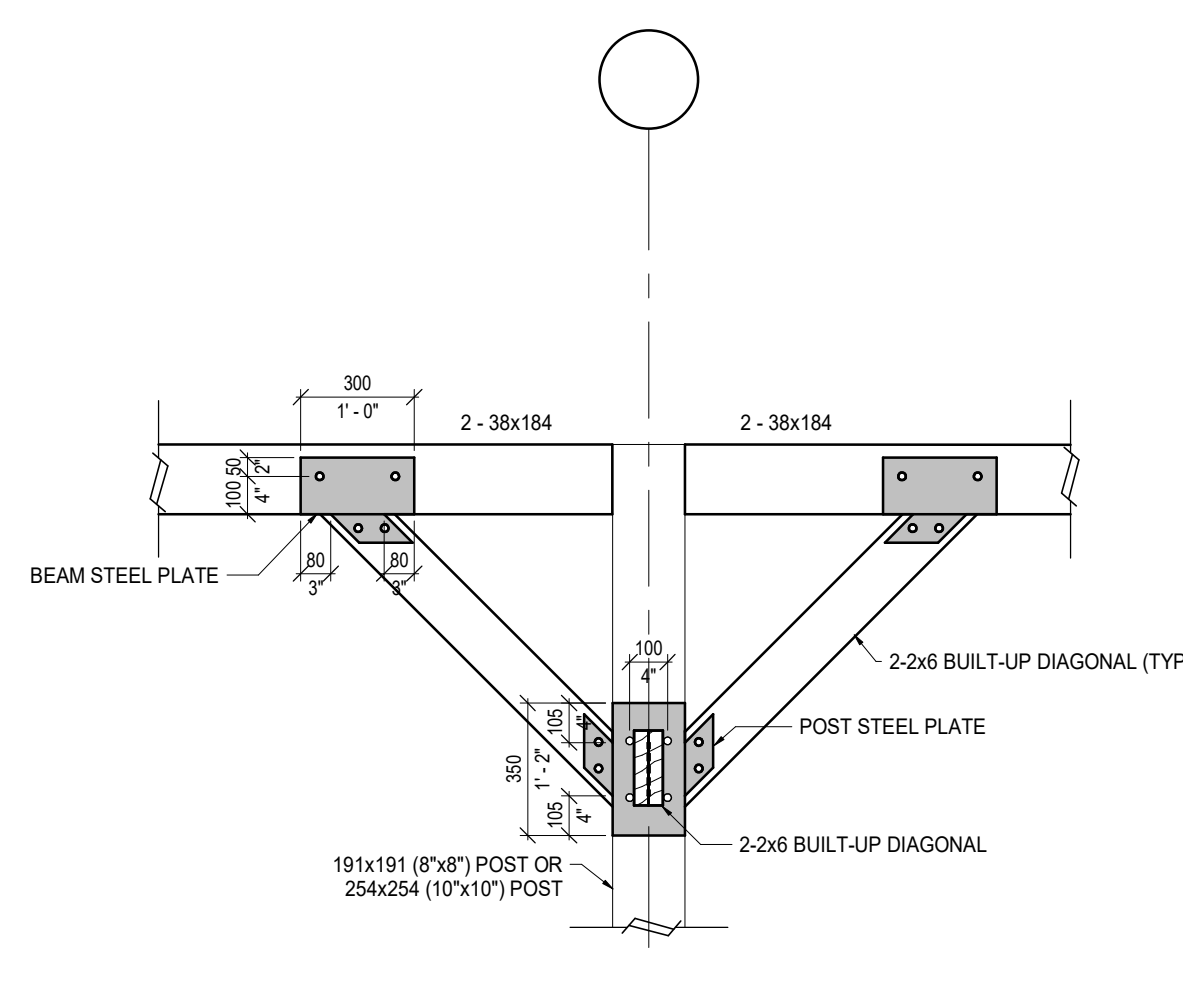
1D POST AND BEAM BRACE STEEL PLATE TYPICAL S402 1 : 20
