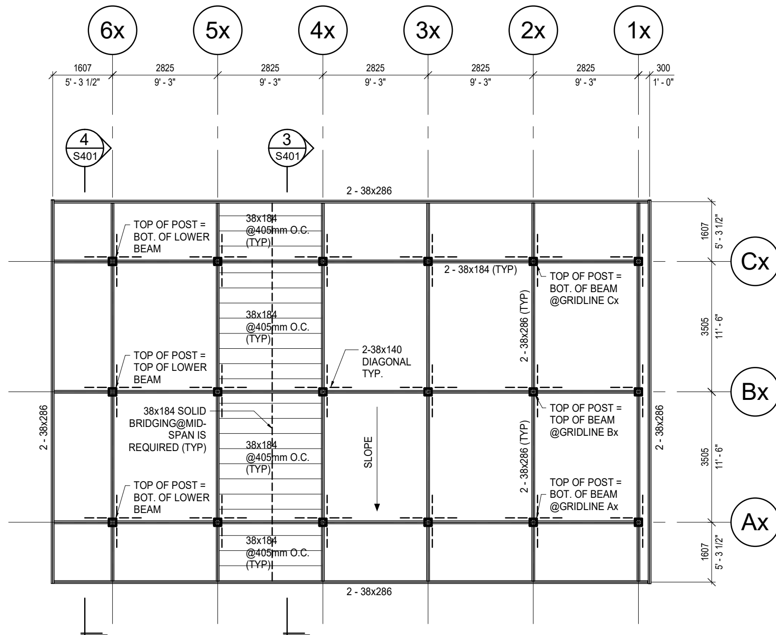
5 ROOF CANOPY 2 S201 1 : 100
