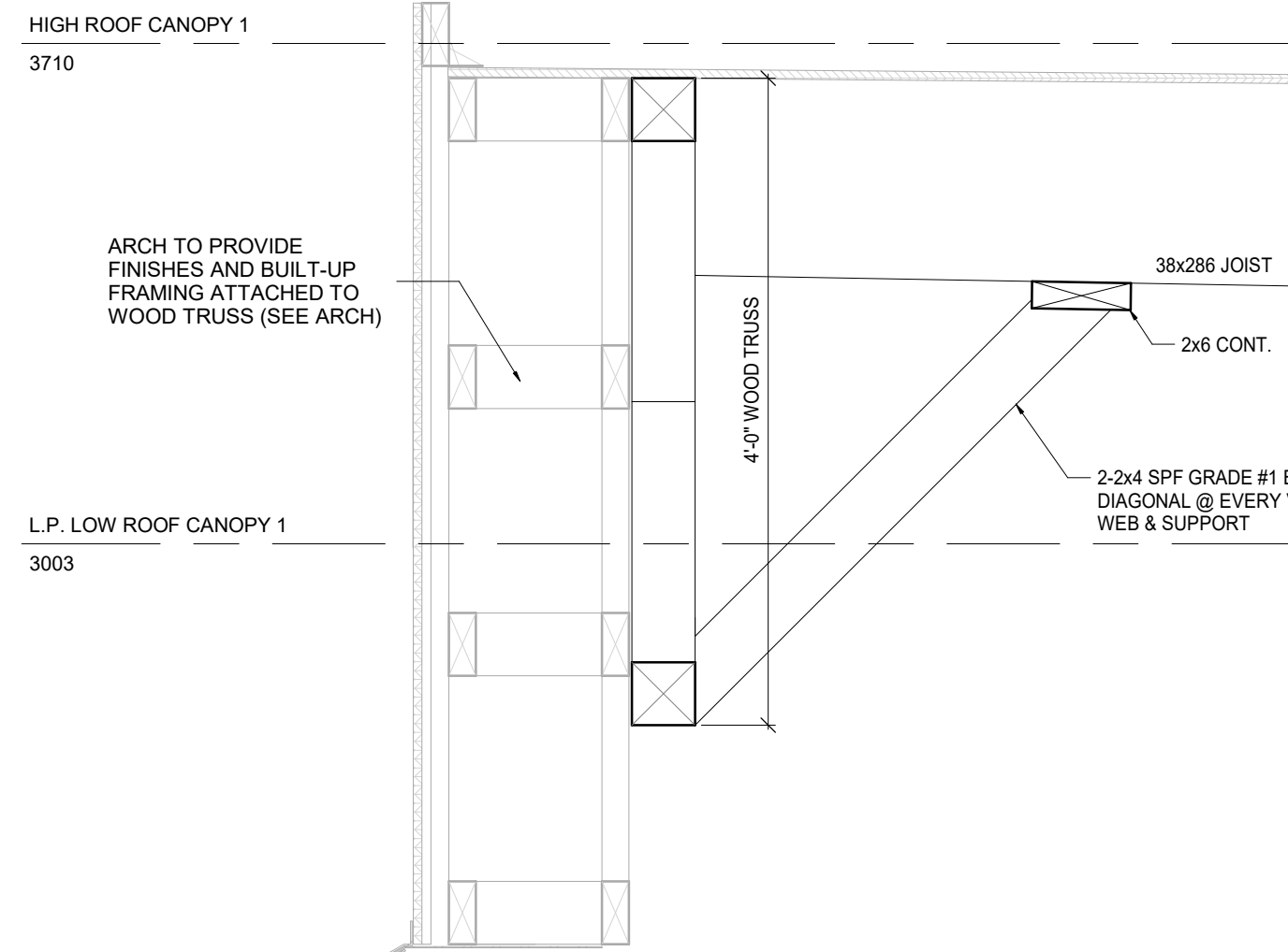
5 SECTION AT WOOD TRUSS S402 1 : 10
