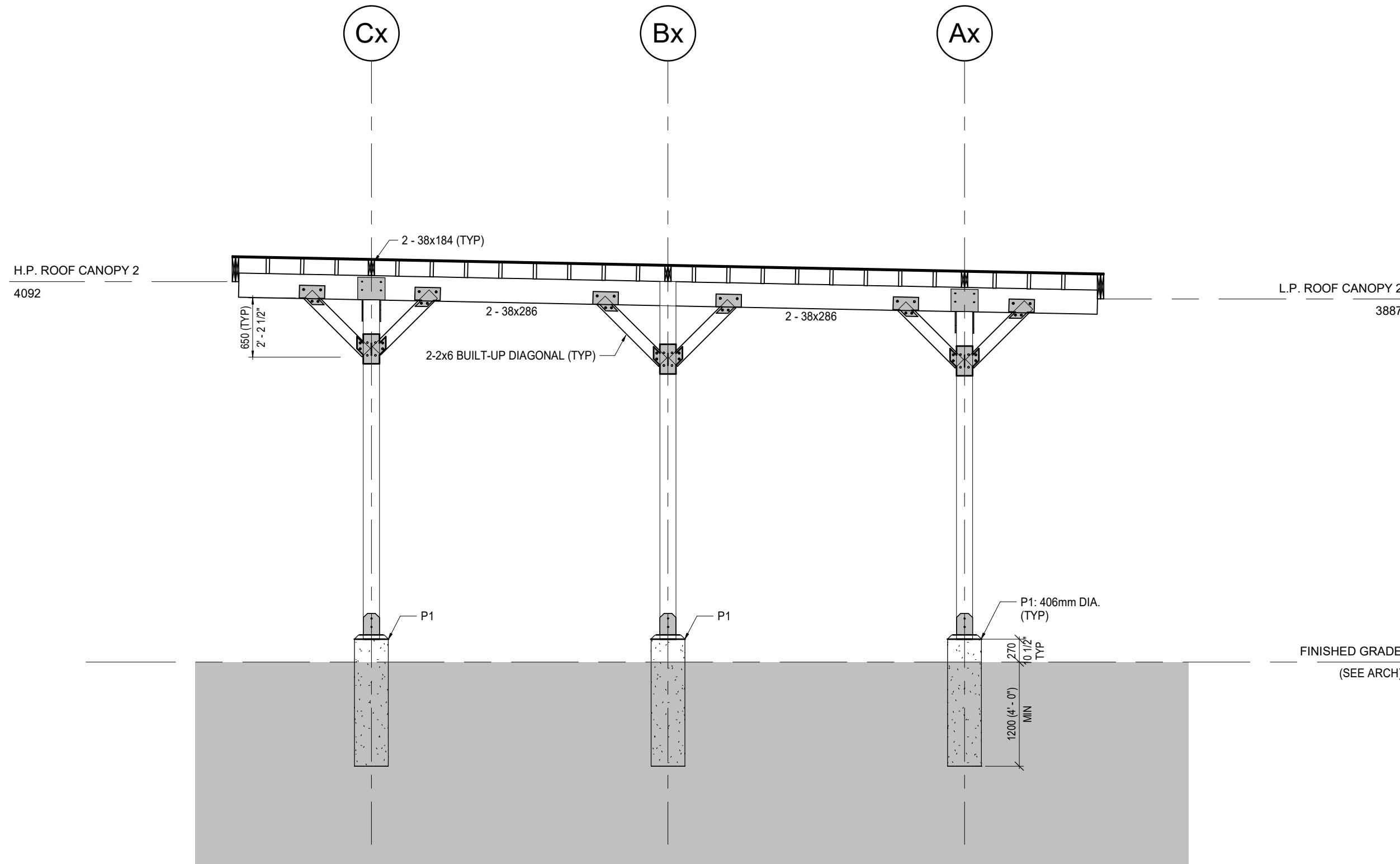
4 SECTION AT G/L 6x S401 1 : 50
