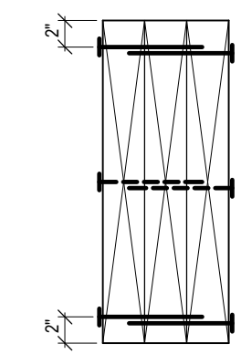
3-PLY WOOD JOIST NAIL ARRANGEMENT 16x(3-12") COMMON WIRE NAIL@12" O.C.
