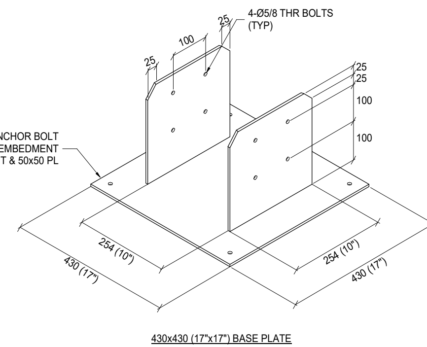
8 BASE PLATE DETAILS S402 1 : 10
