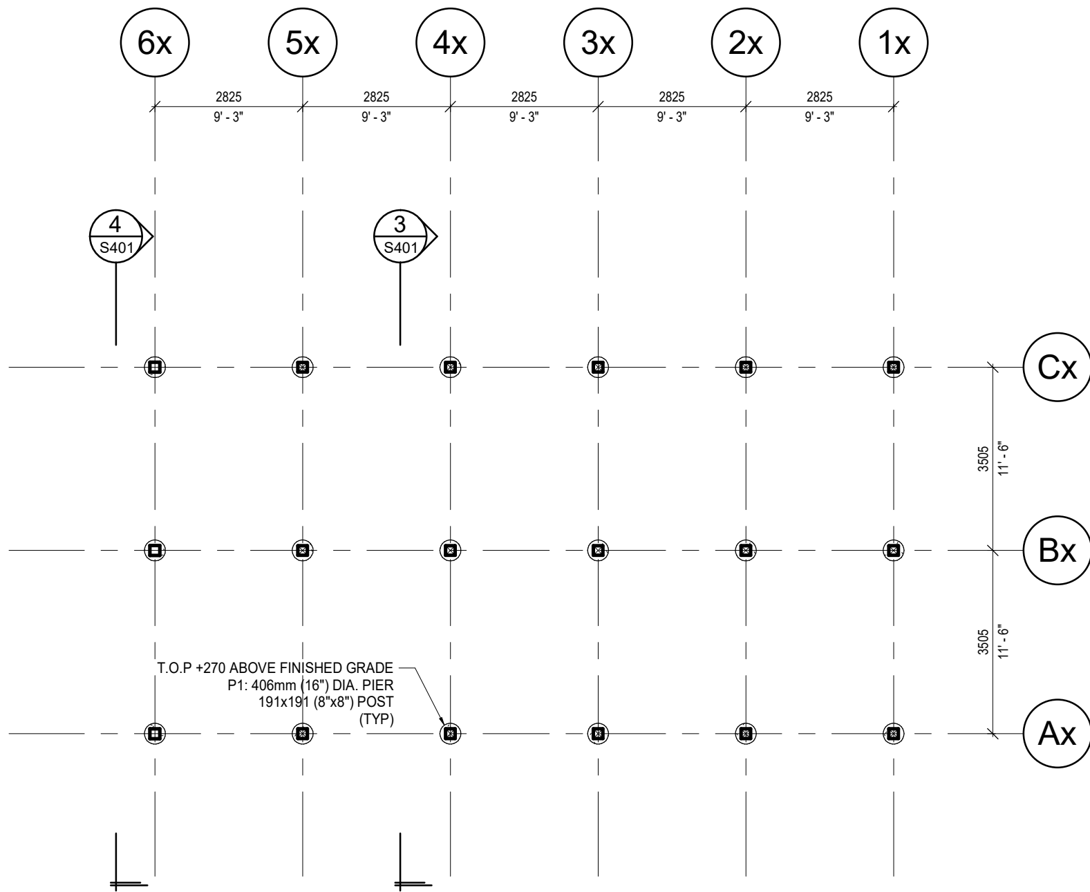
4 GROUND FLOOR CANOPY 2 S201 1 : 100
