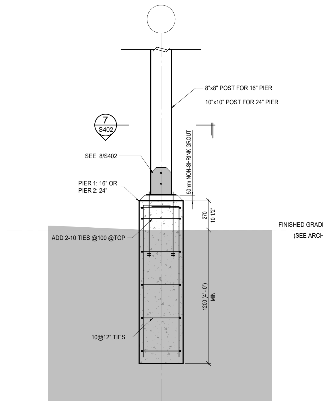
6 CONCRETE PIER & POST ELEVATION (TYPICAL) S402 1 : 20
