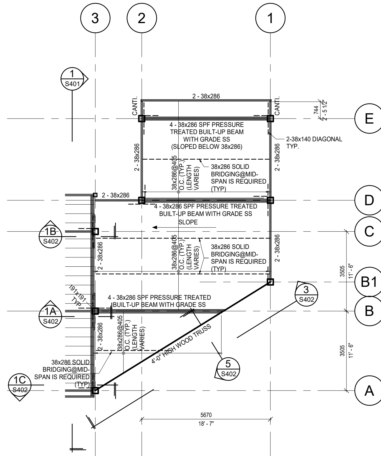
3 HIGH ROOF CANOPY 1 S201 1 : 100
