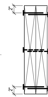
2-PLY WOOD JOIST NAIL ARRANGEMENT 10x(3") COMMON WIRE NAIL@12" O.C.
