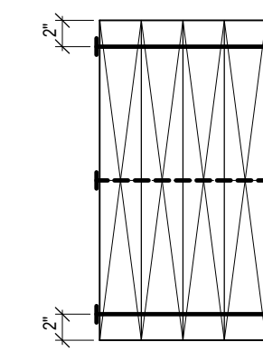
4-PLY OR 5-PLY WOOD JOIST NAIL CONNECTION 1/2" A307 THROUGH BOLTS @ 12" O.C.
