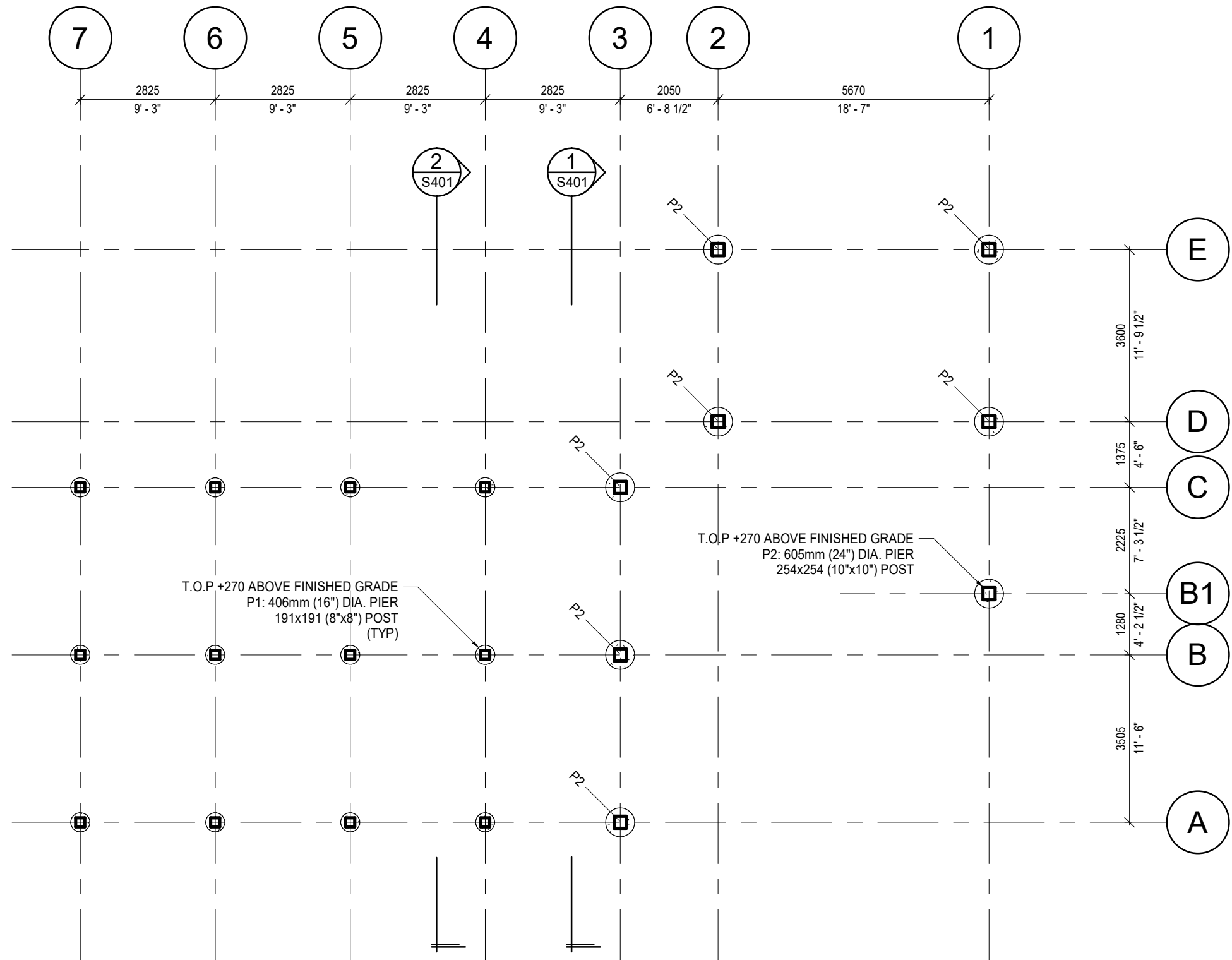
1 GROUND FLOOR CANOPY 1 S201 1 : 100
